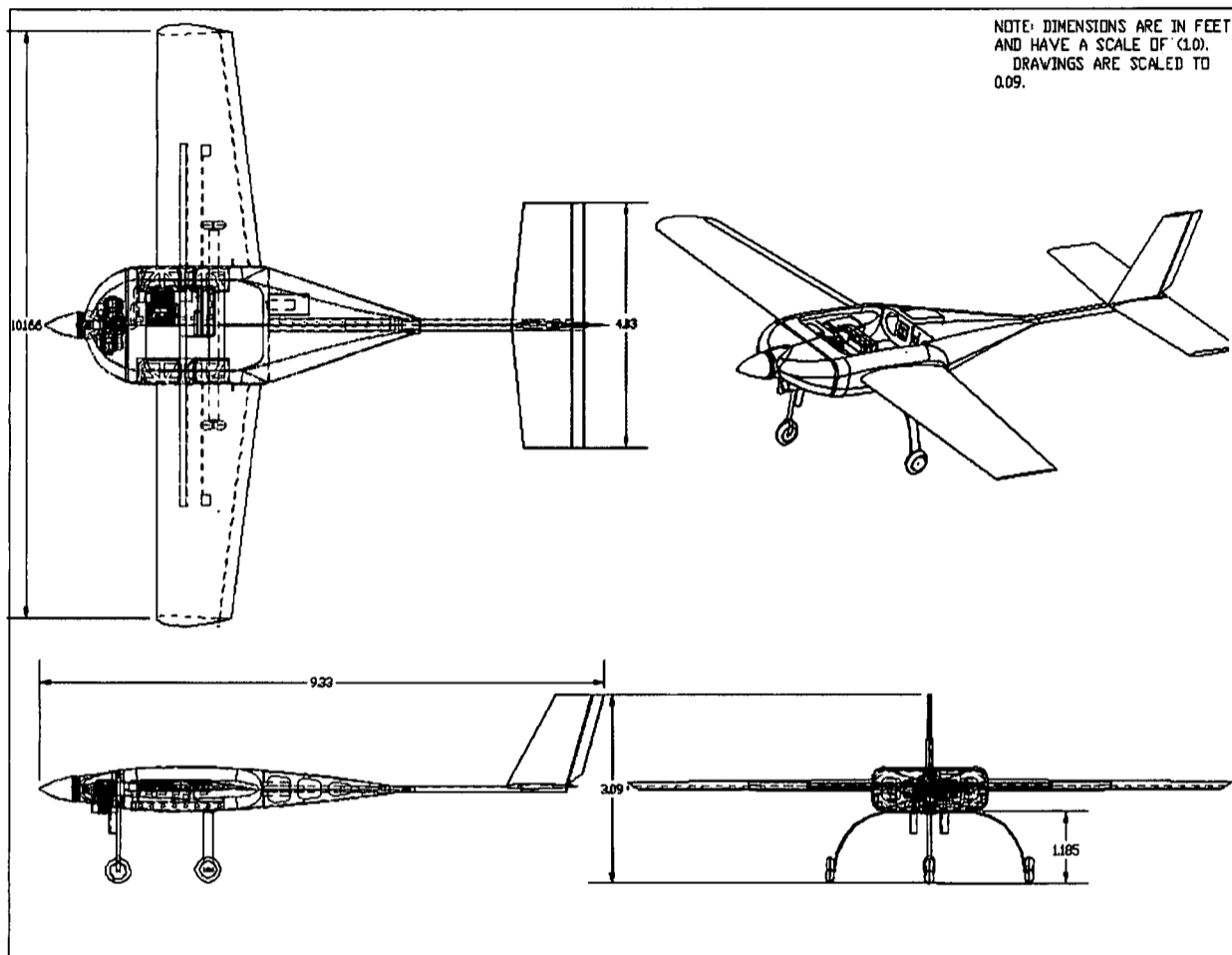
Figure: 6 Cobra 3 View Drawing
